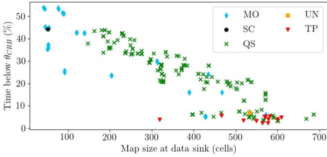
Fig. 3. Average percent of time spent with CRB below \theta_{CRB} per robot against number of map cells known at data sink for 4 robots in 30x30 space with 20 obstacles. Each point is the average performance of 6 trials, and ideal is at the top right. We show more points for the more parameterized approaches (MO and our novel QS), while SC and UN are captured by a single point because they do not depend on parameters.
